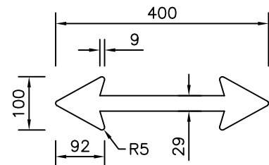
ARROW DETAIL Scale 1:10
